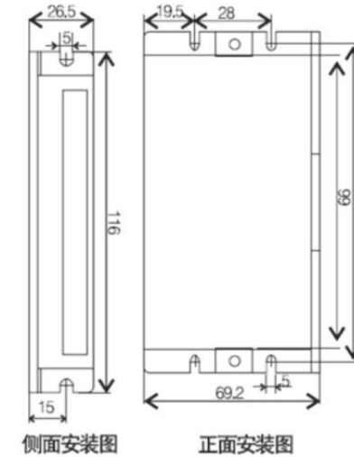
Figure 1: Installation specifications
