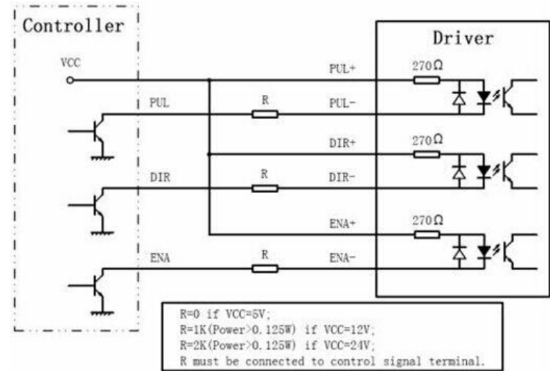
Figure 2: Connections to open-collector signal (common-anode)
